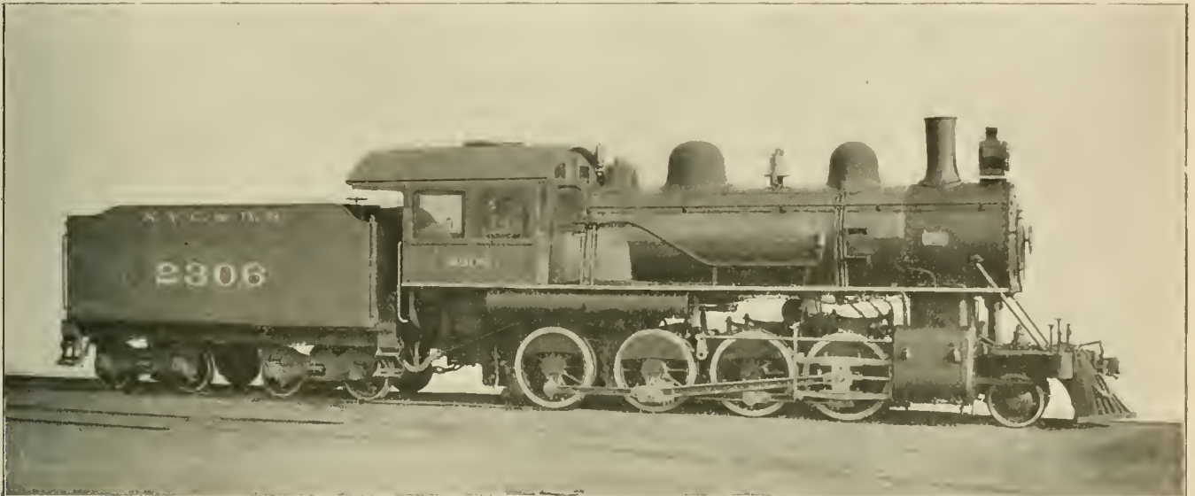
CROSS-COMPOUND CONSOLIDATION FOR THE NEW YORK CENTRAL.
